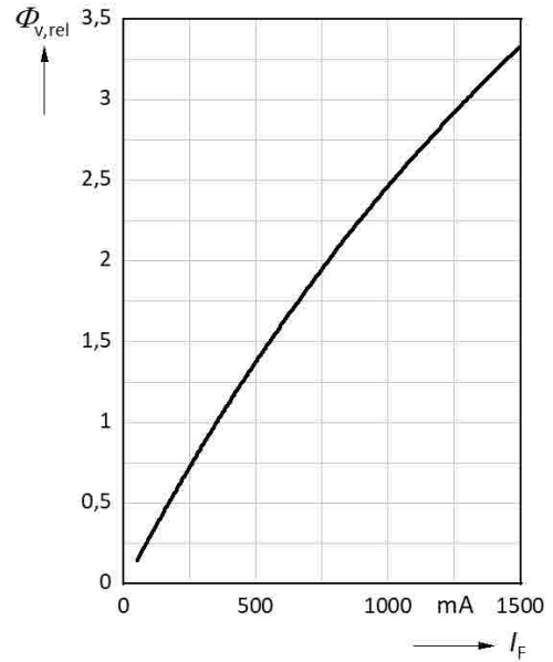
Relative Luminous Flux vs. Forward Current
