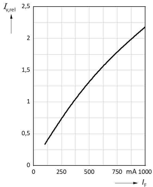
Relative Luminous Intensity vs. Forward Current
