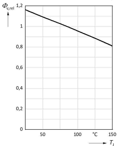
Relative Luminous Flux vs. Junction Temperature
