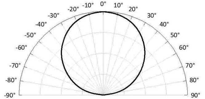
Radiation Pattern
