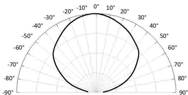
Radiation Pattern
