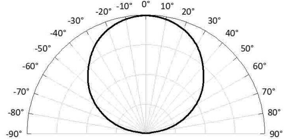
Radiation Pattern
