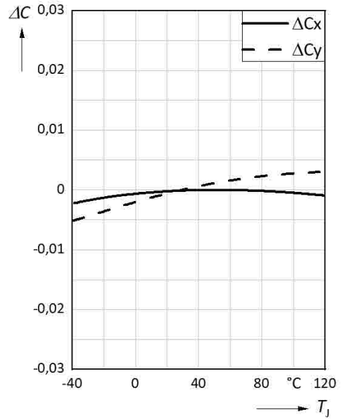
Chromaticity Shift vs. Junction Temperature
