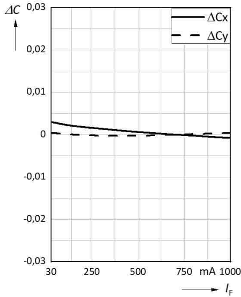
Chromaticity Shift vs. Forward Current
